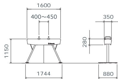
AF020M41 Pommel for Spare
